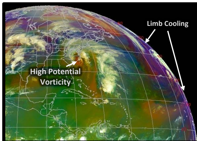
Air Mass RGB from GOES-16 at 1445 UTC, 25 April 2017
